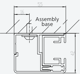
Wall mounting
