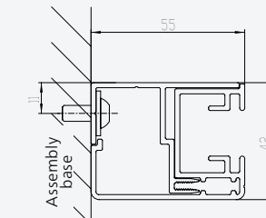
Installation in reveals
